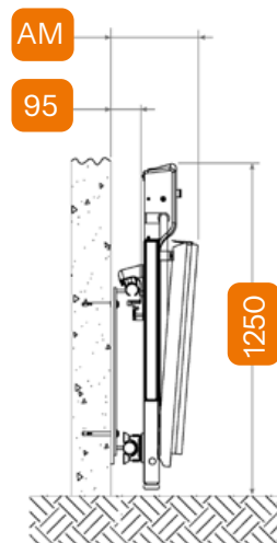
Folded platform, wall fixation
