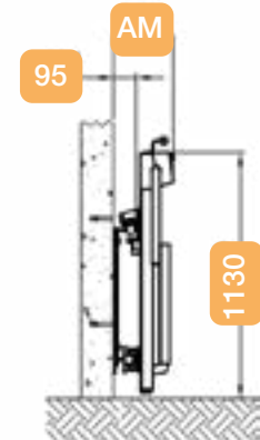
Folded platform, wall fixation
