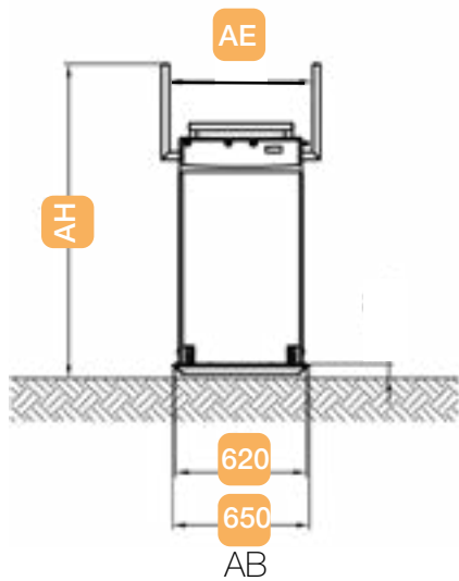
Unfolded platform (loading/ unloading at the bottom floor)
