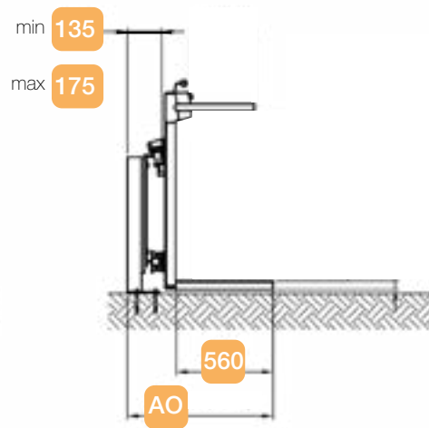
Unfolded platform, fixation with legs
